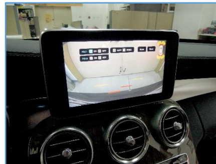
③ Adjust PDC sensors position and ON / OFF
